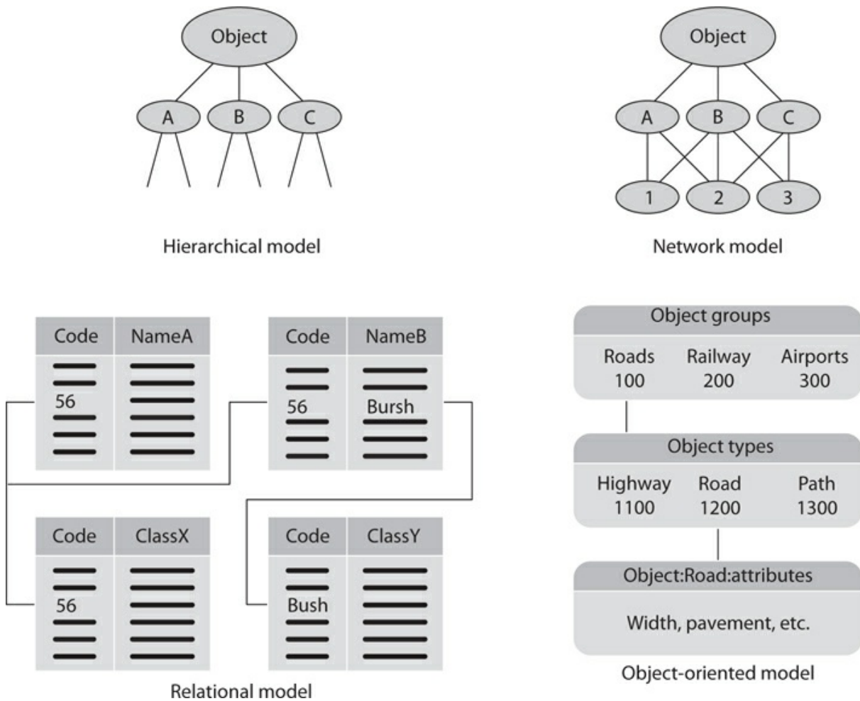
Figure 8-34 Various database models
