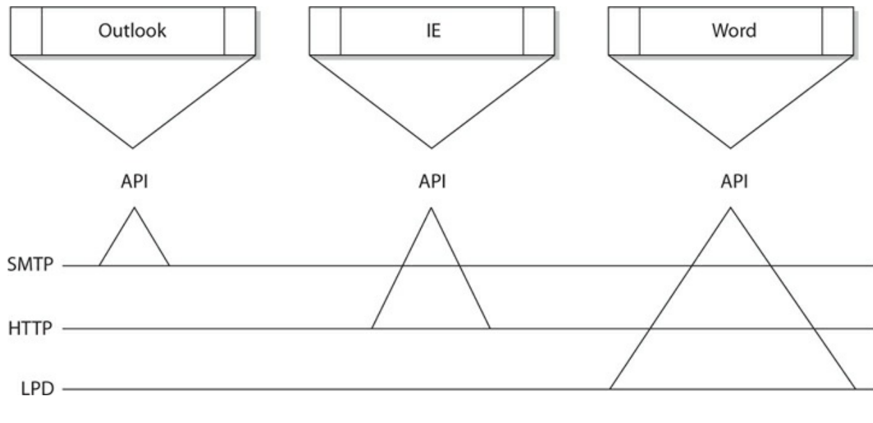
Figure 4-3 Applications send requests to an API, which is the interface to the supporting protocol.
