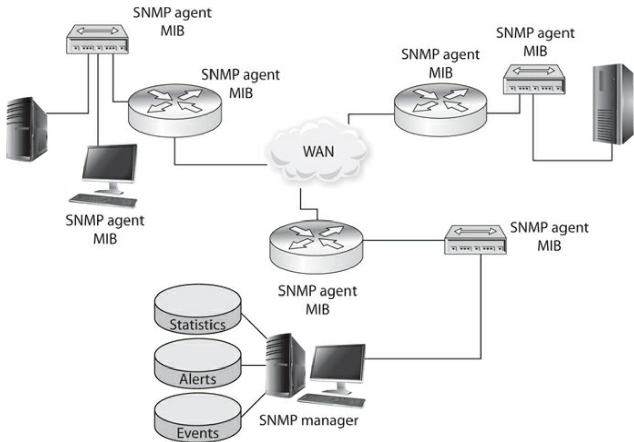
Figure 4-33 Agents provide the manager with SNMP data.
