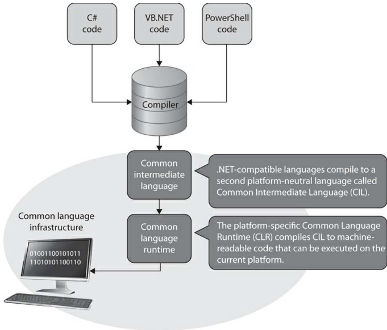
Figure 8-25 .NET Framework components
