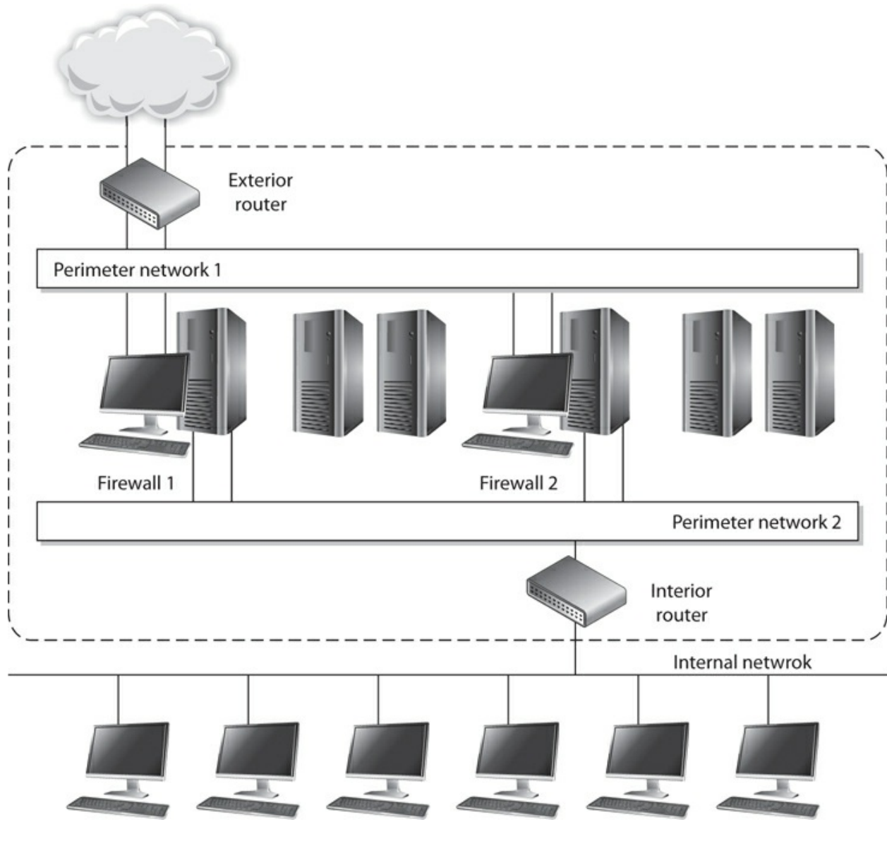
Figure 4-52 A screened subnet can have different networks within it and different firewalls that filter for specific threats.
