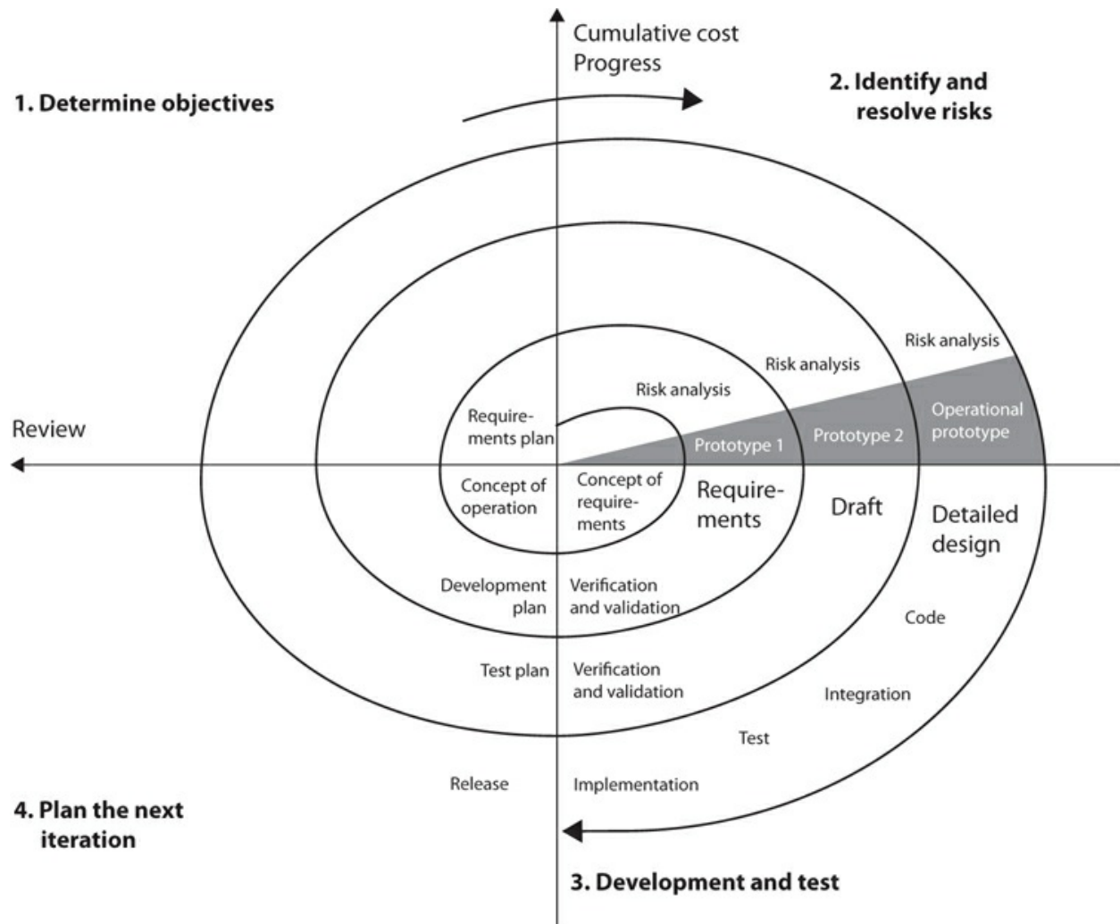
Figure 8-10 Spiral model for software development
