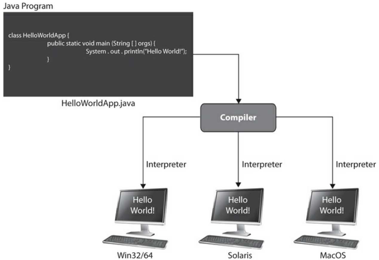
Figure 8-13 Java bytecode is converted by interpreters.
