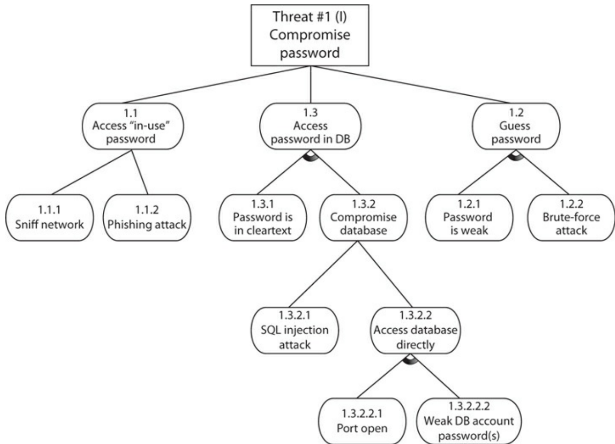
Figure 8-4 Threat tree used in threat modeling
