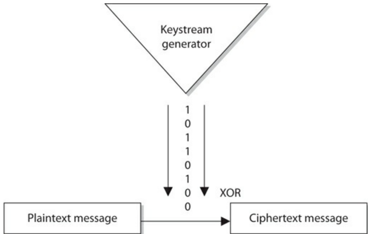
Figure 3-35 With stream ciphers, the bits generated by the keystream generator are XORed with the bits of the plaintext message.
