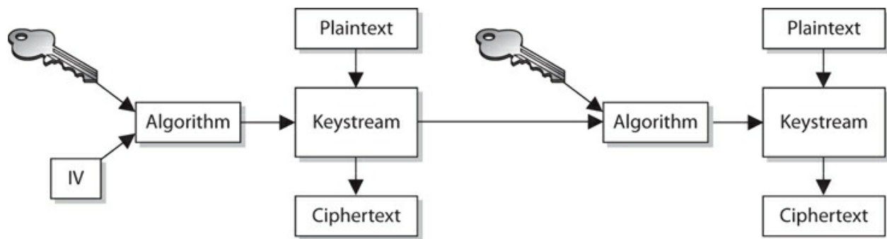
Figure 3-41 A block cipher working in OFB mode
