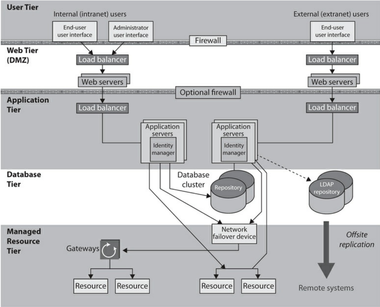
Figure 7-17 High-availability technologies
