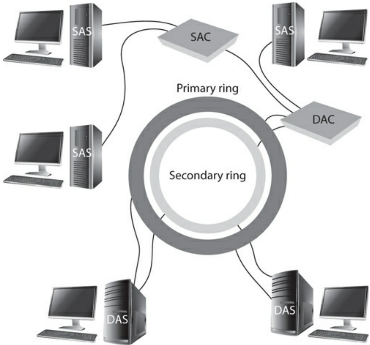
Figure 4-30 FDDI device types
