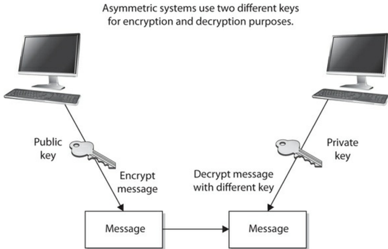
Figure 3-33 An asymmetric cryptosystem
