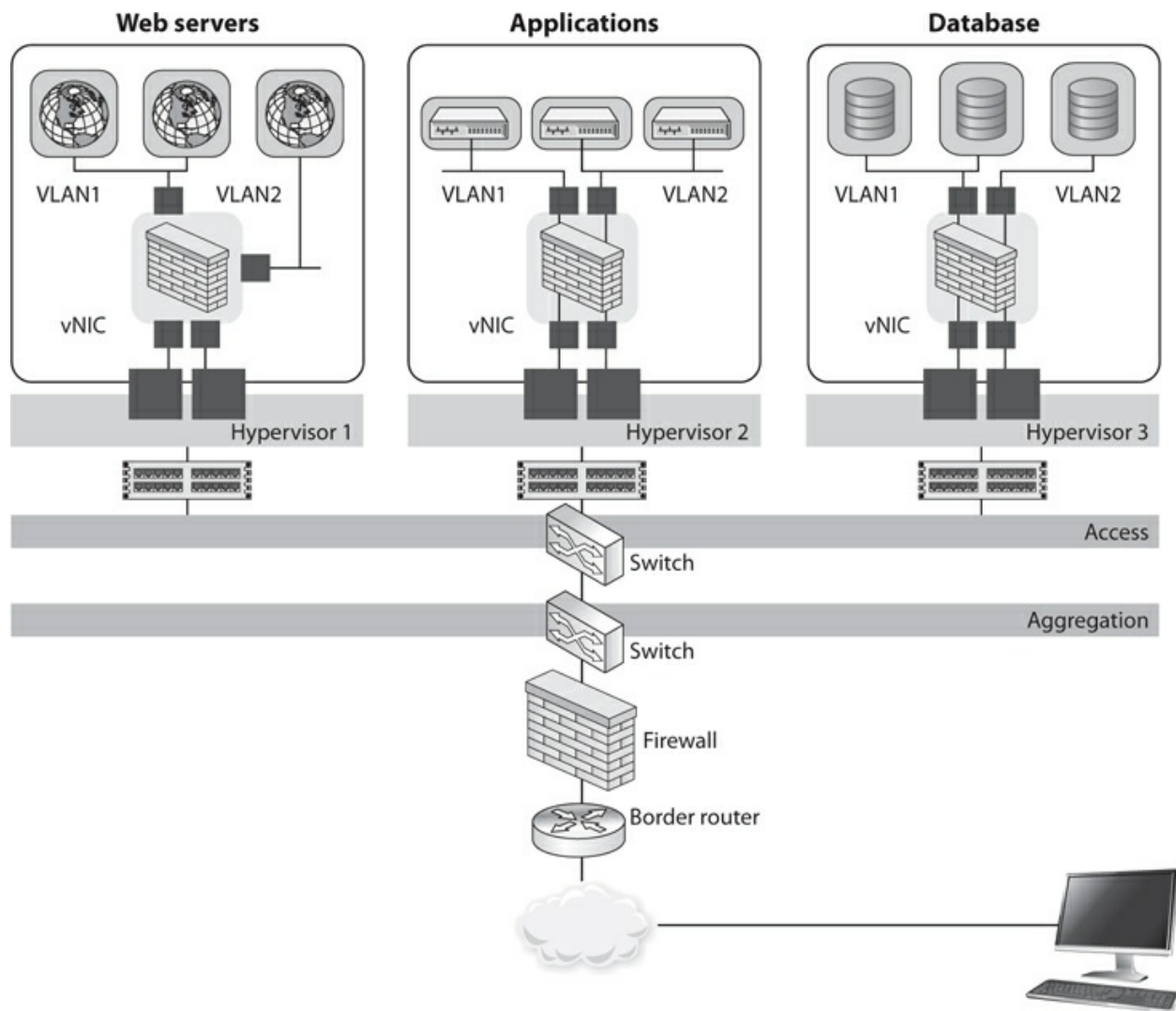
Figure 4-54 Virtual firewalls
