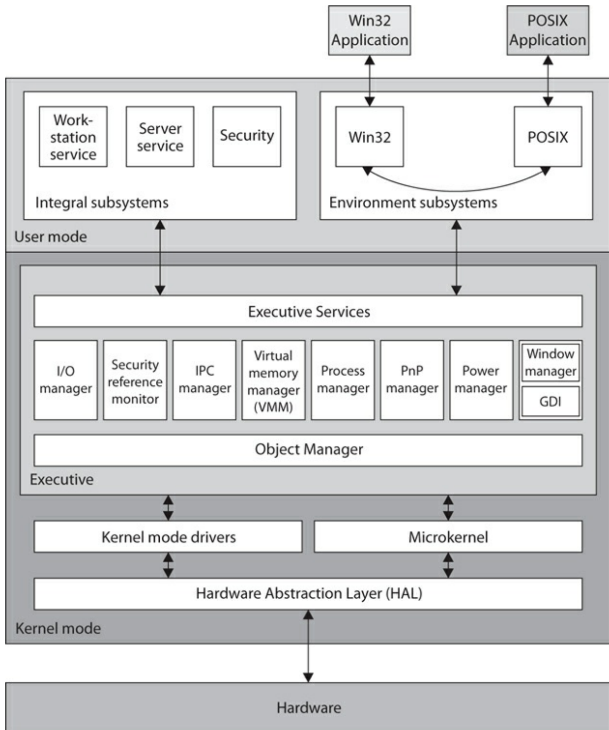
Figure 3-19 Windows hybrid microkernel architecture
