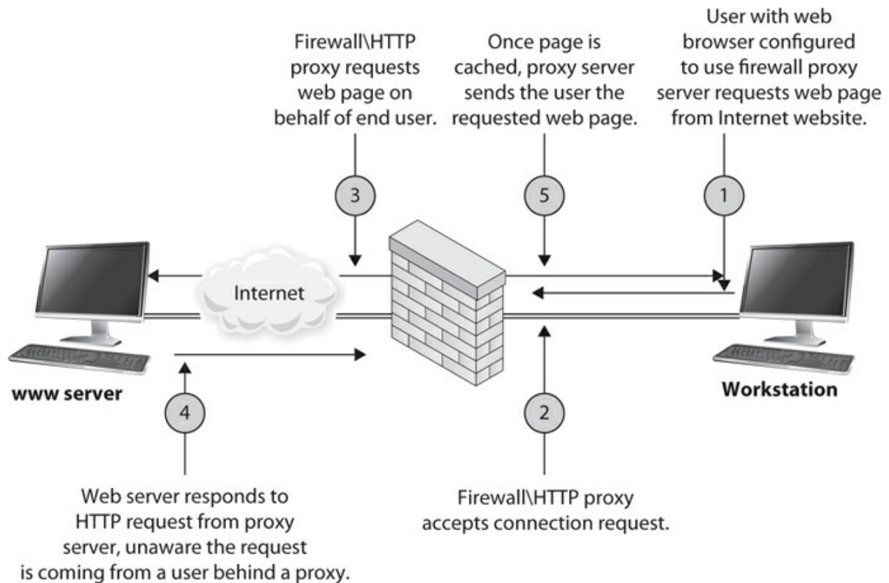
Figure 4-47 Proxy firewall breaks connection
