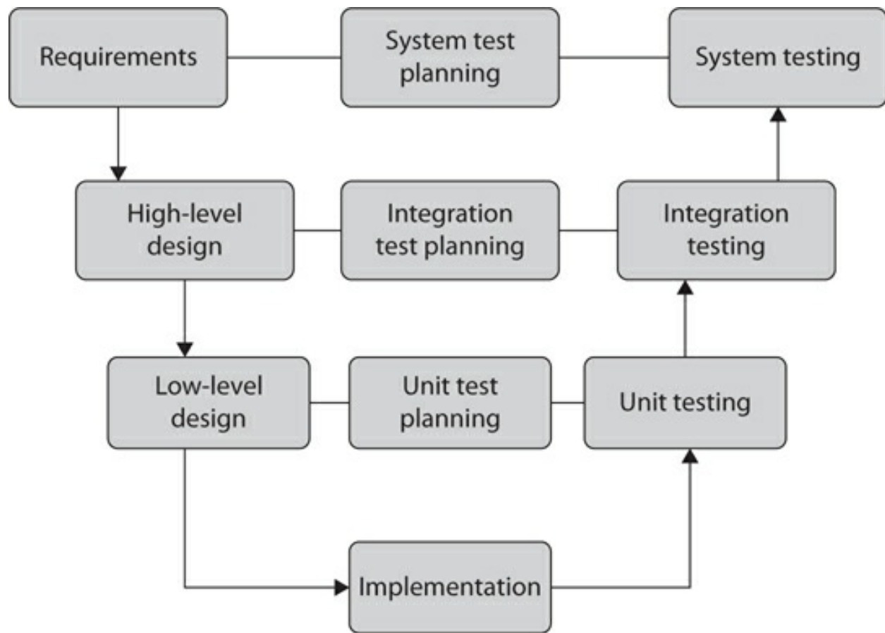
Figure 8-8 V-shaped model
