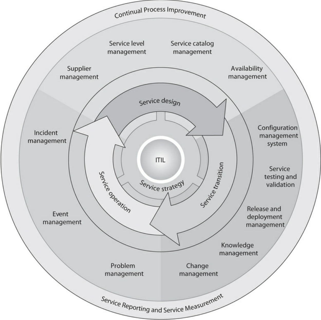
Figure 1-6 ITIL
