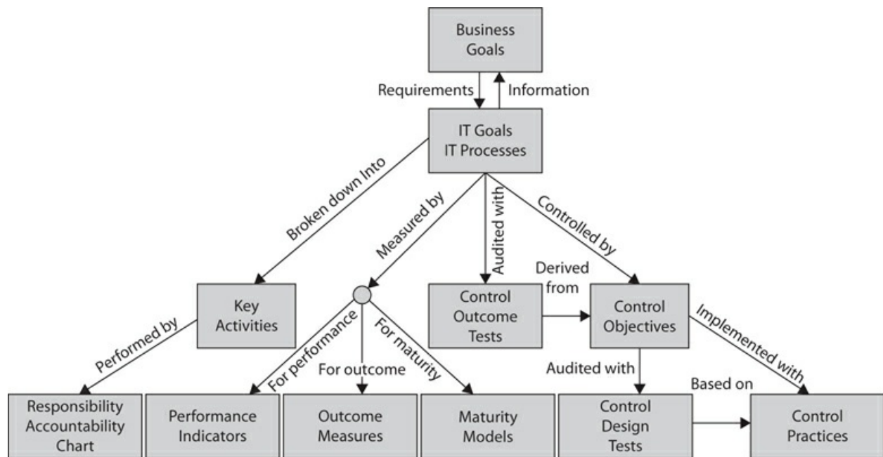
Figure 1-5 COBIT framework
