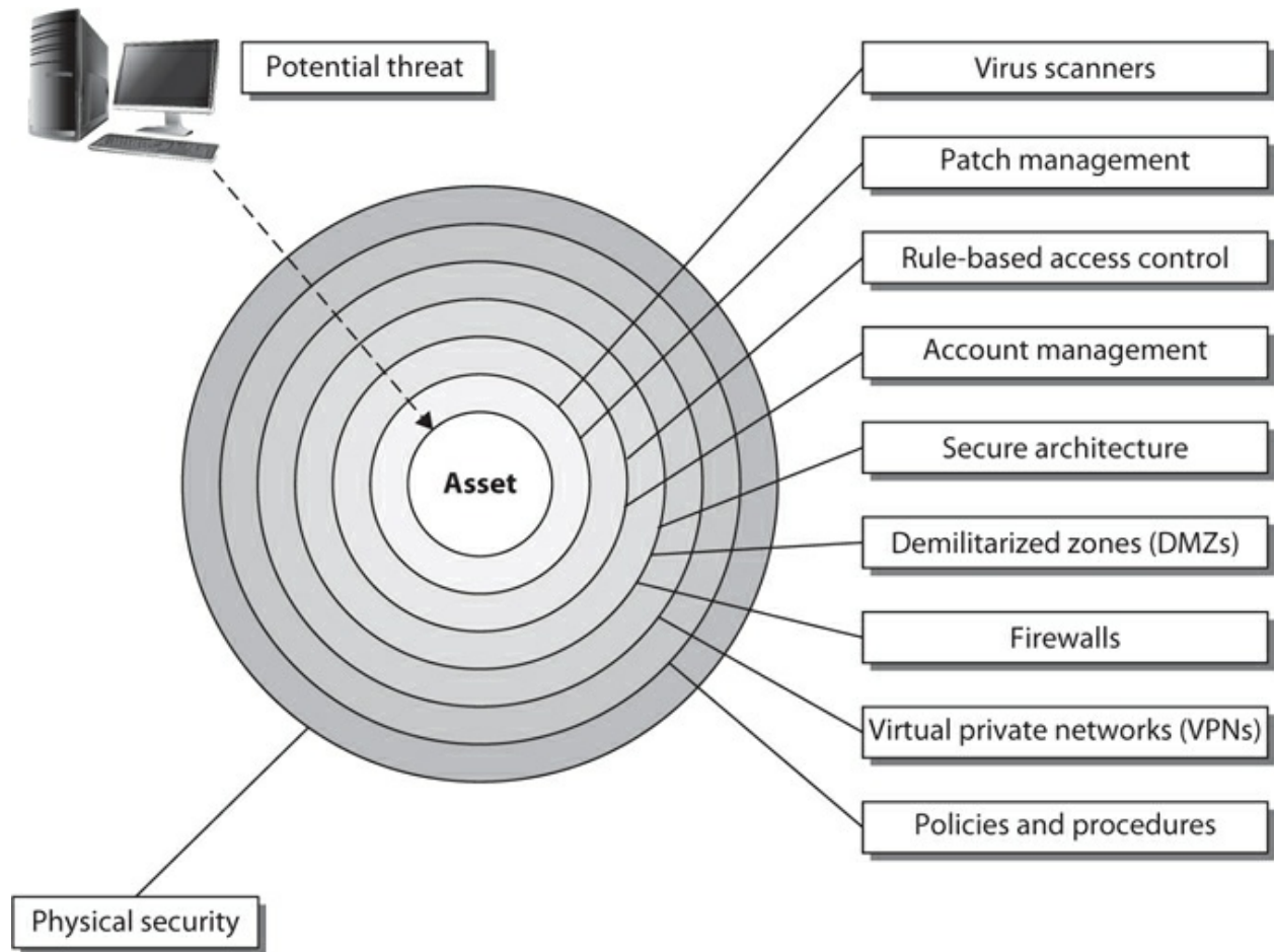
Figure 1-2 Defense-in-depth
