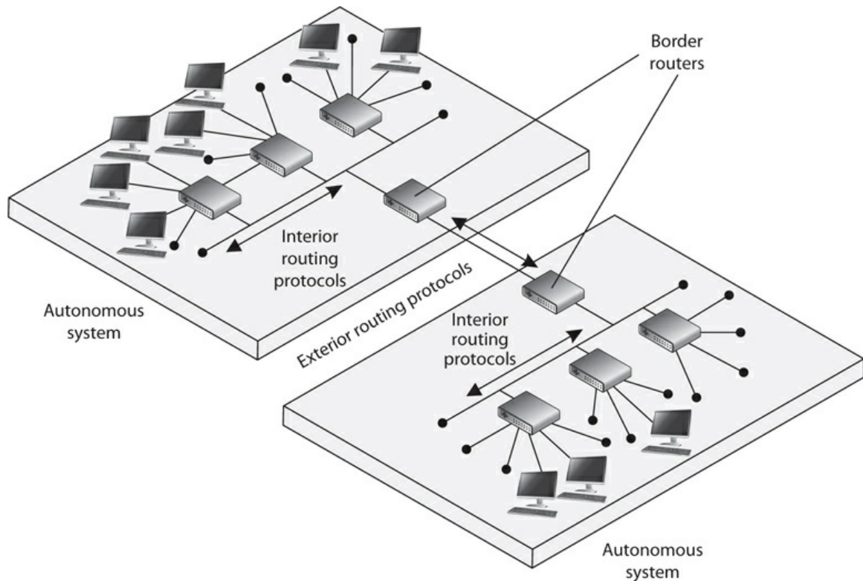
Figure 4-37 Autonomous systems
