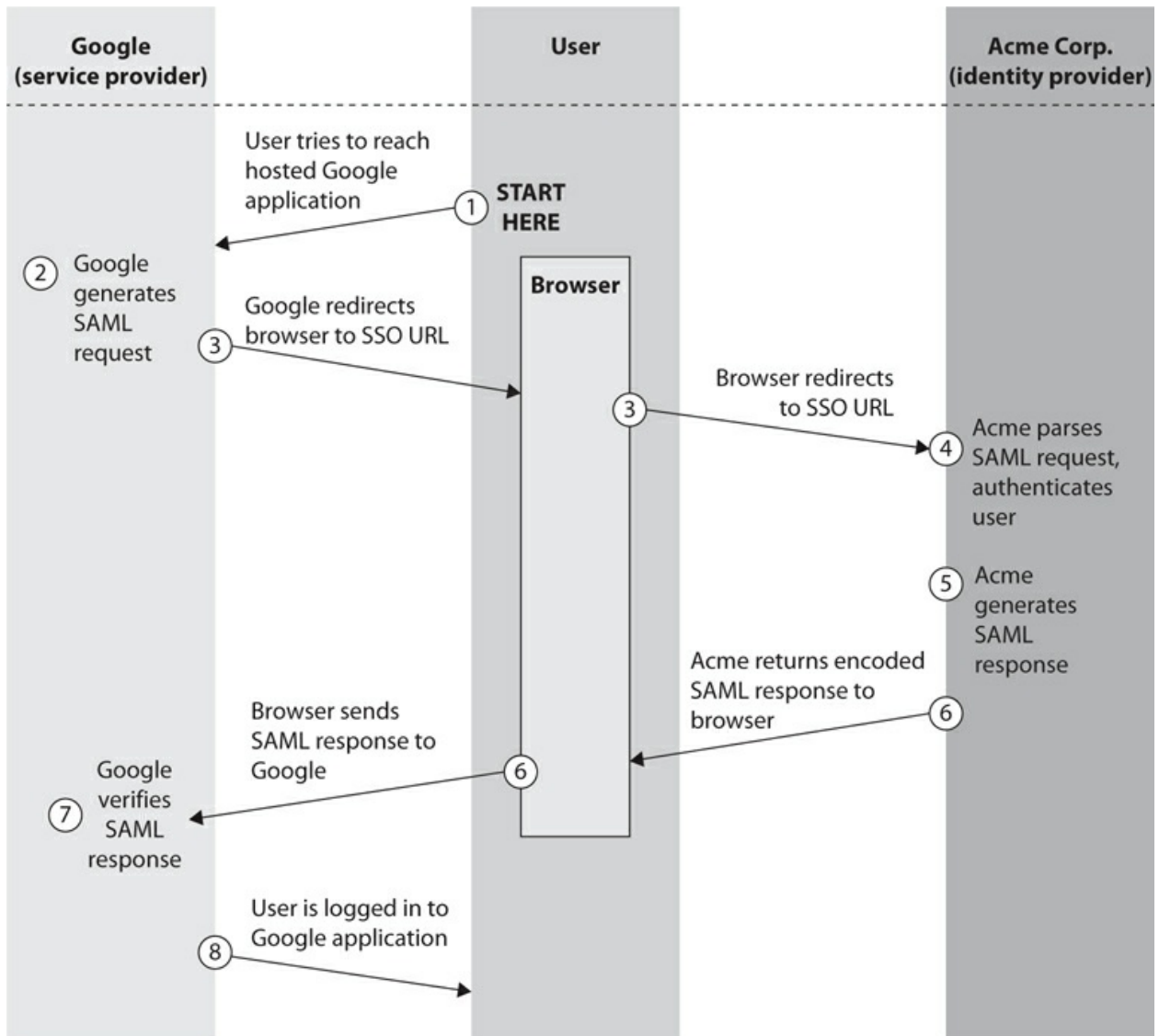
Figure 5-14 SAML authentication
