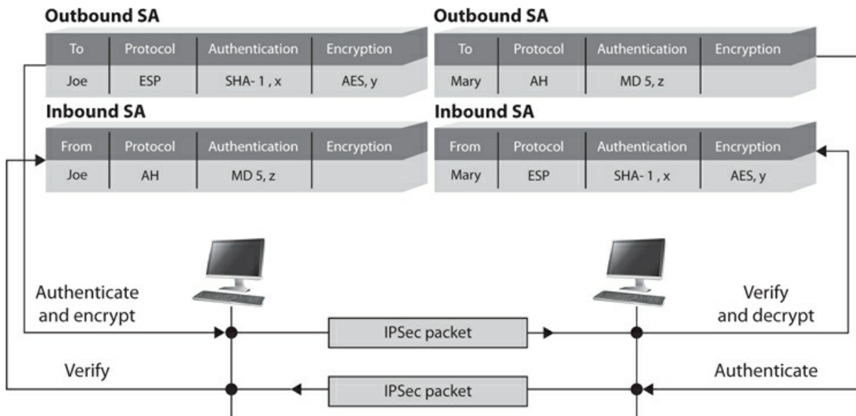
Figure 4-72 IPsec uses security associations to store VPN parameters.
