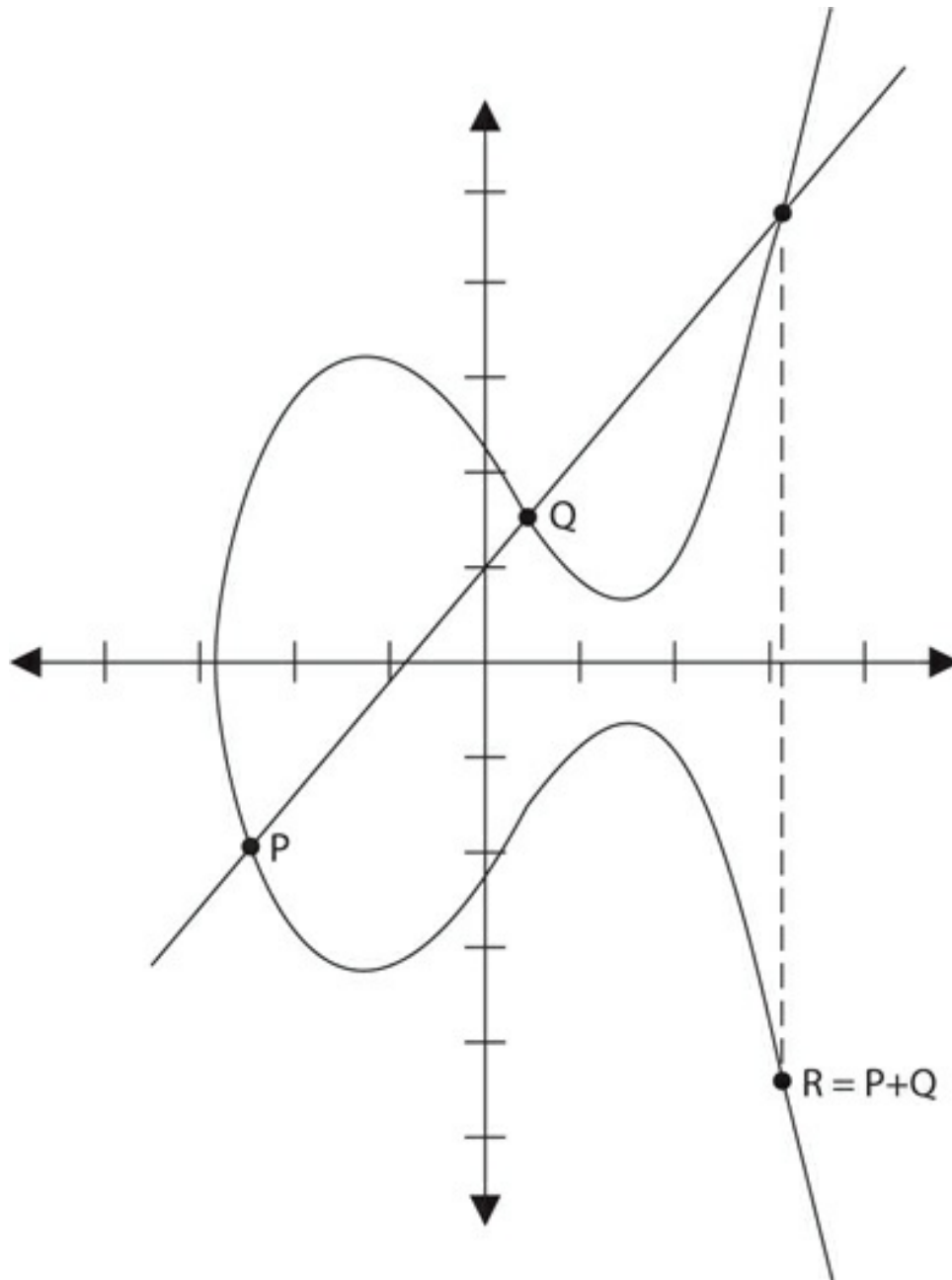
Figure 3-43 Elliptic curve
