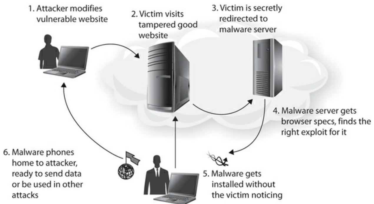
Figure 6-7 Drive-by downloads
