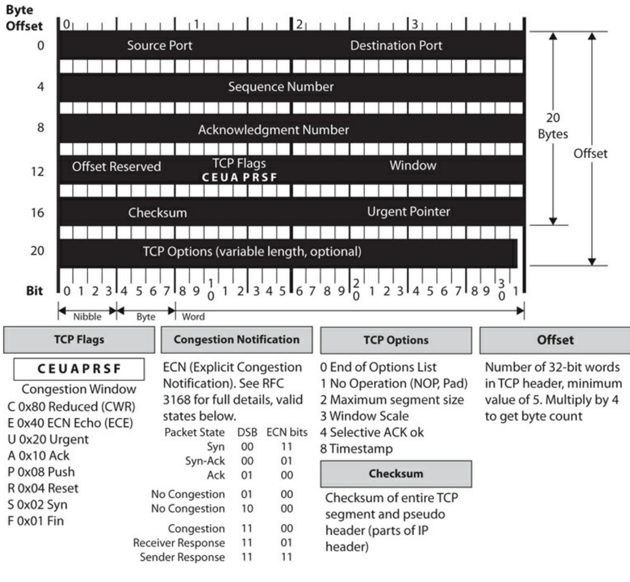
Figure 4-46 TCP header
