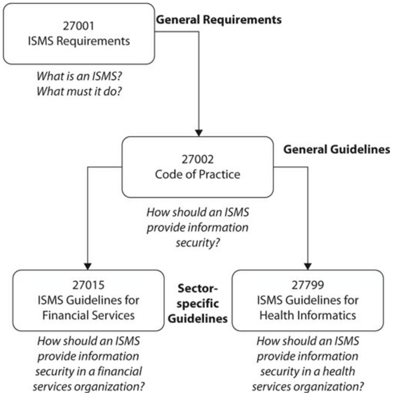
Figure 1-3 ISO/IEC 27000 standards
