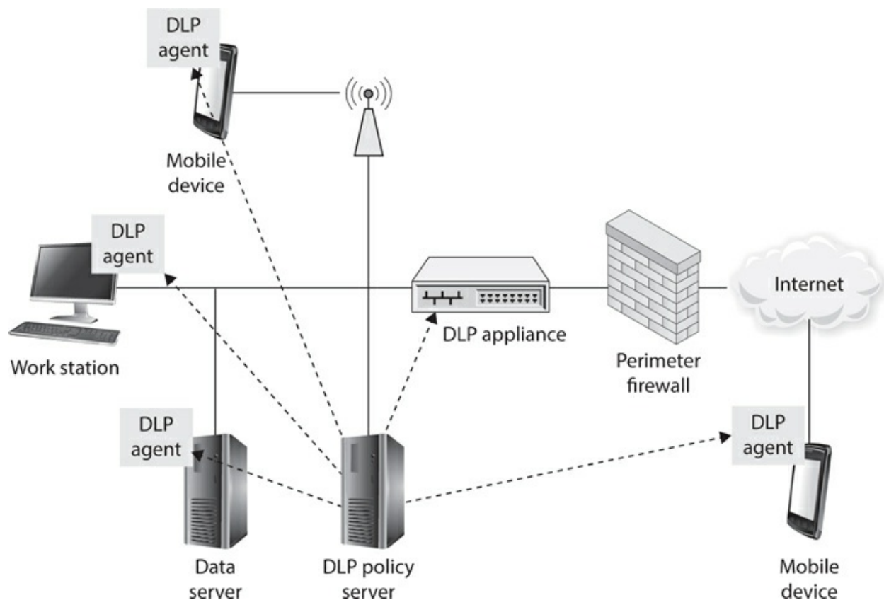
Figure 2-9 Hybrid NDLP/EDLP
