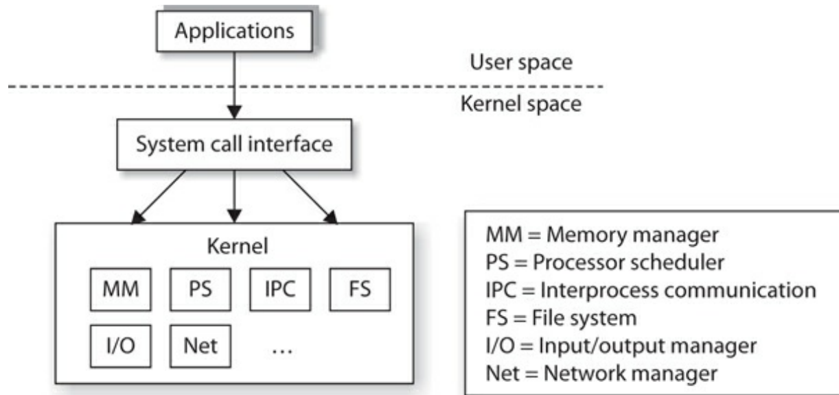
Figure 3-16 Monolithic operating system architecture
