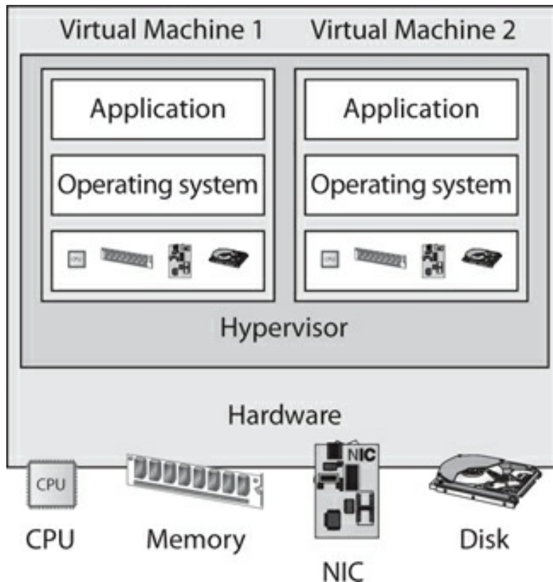
Figure 3-21 The hypervisor controls virtual machine instances.
