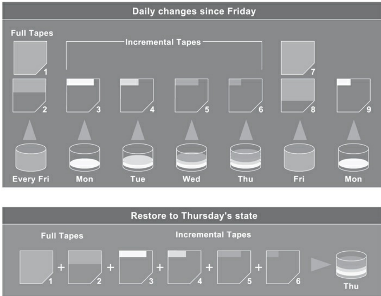
Figure 7-14 Backup software steps
