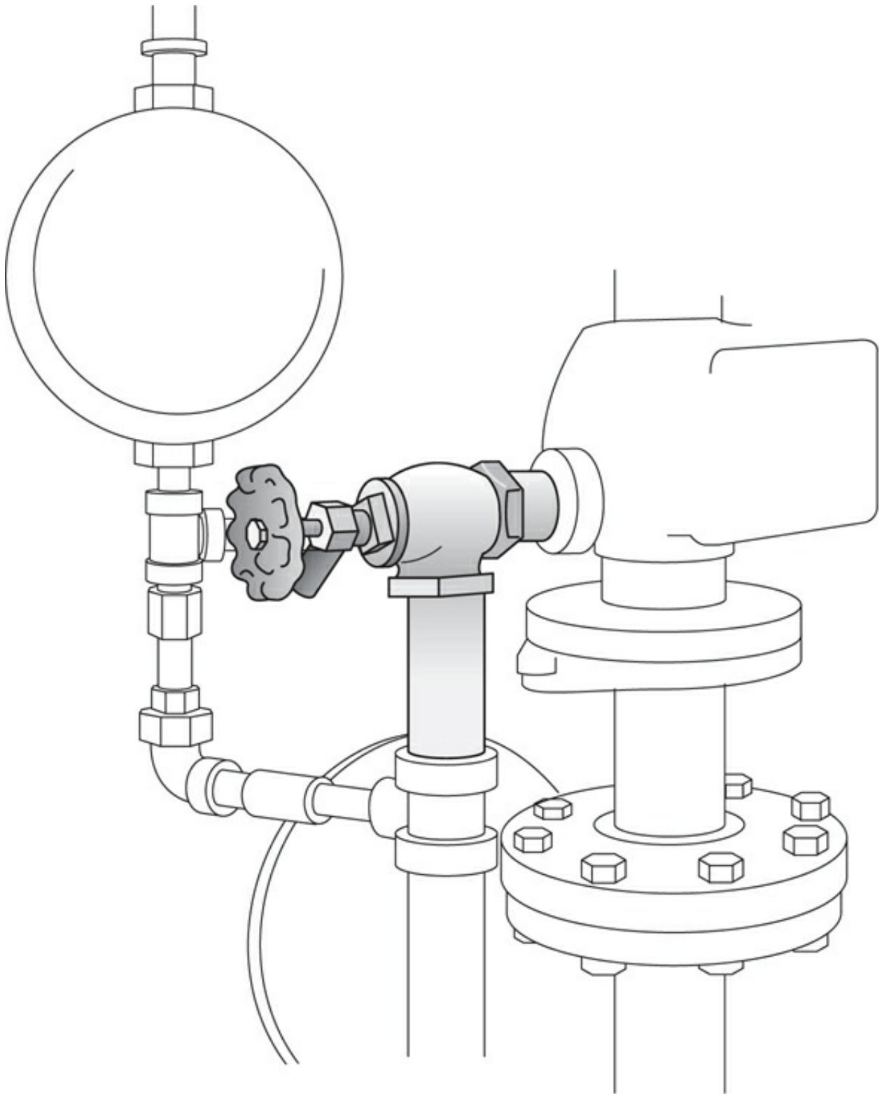
Figure 3-57 Water, steam, and gas lines should have emergency shutoff valves.
