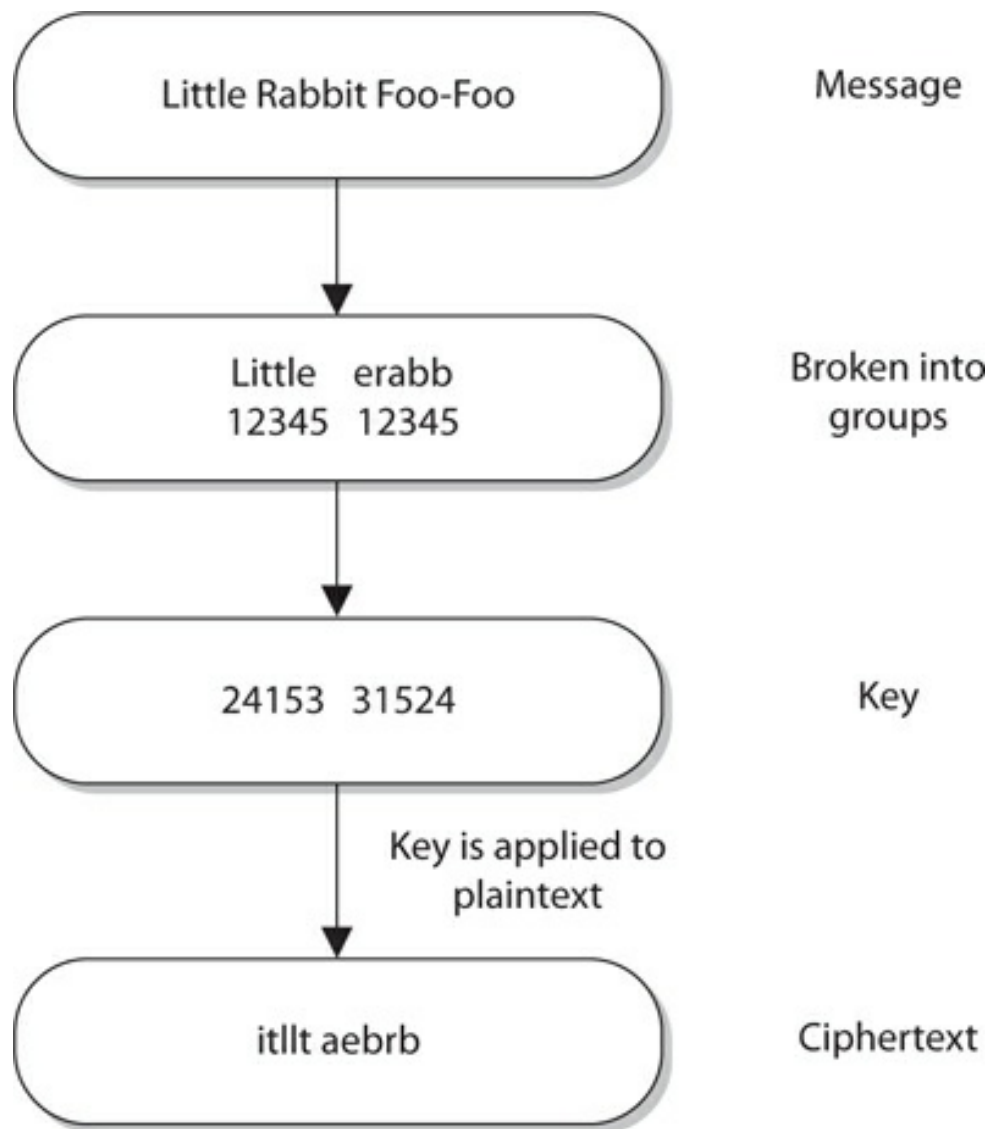
Figure 3-30 A transposition cipher
