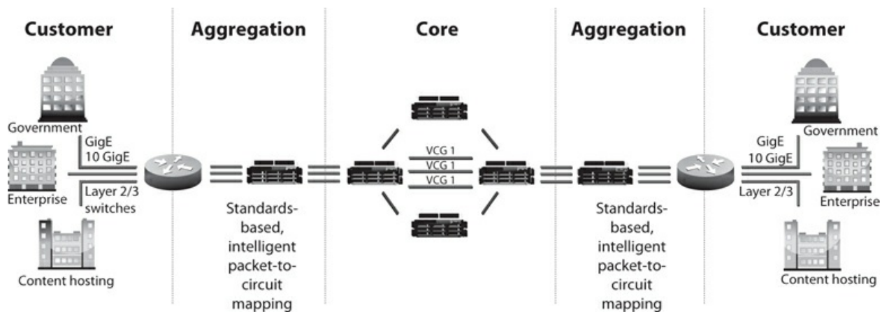
Figure 4-60 MAN architecture
