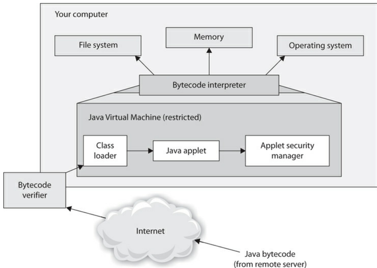
Figure 8-29 Java's security model
