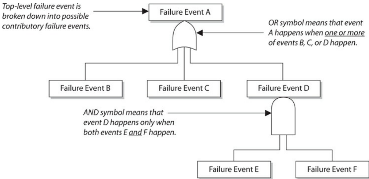
Figure 1-15 Fault tree and logic components
