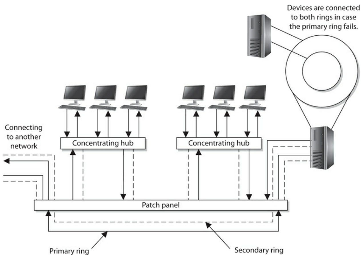
Figure 4-29 FDDI rings can be used as backbones to connect different LANs.
