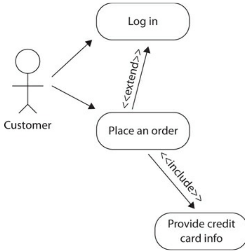
Figure 6-3 UML use case diagram
