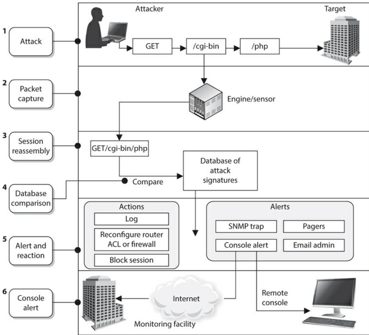
Figure 5-24 The basic architecture of a NIDS
