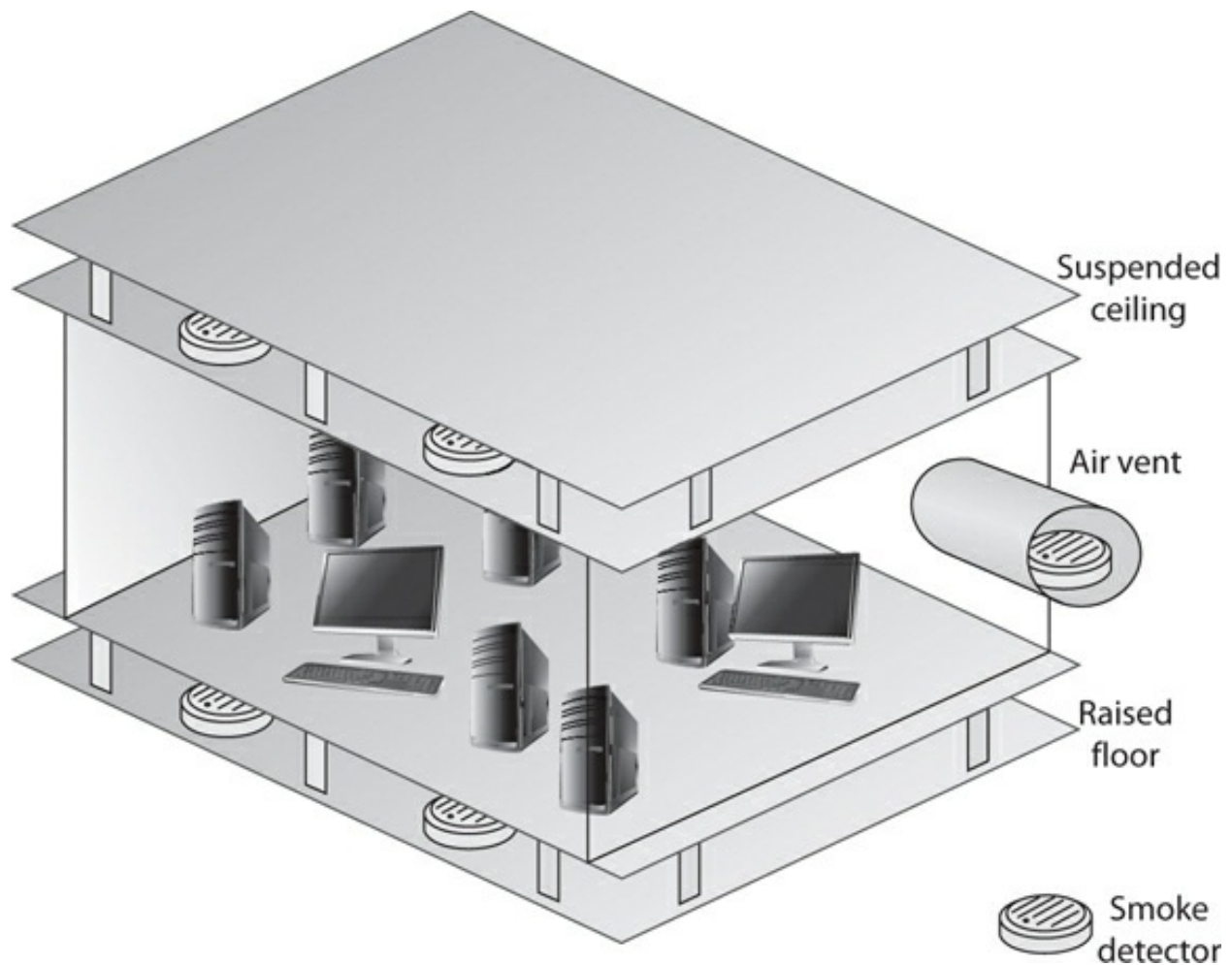
Figure 3-60 Smoke detectors should be located above suspended ceilings, below raised floors, and in air vents.
