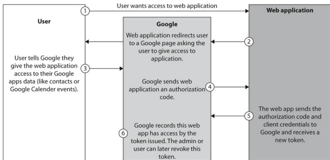
Figure 5-16 OAuth authorization steps
