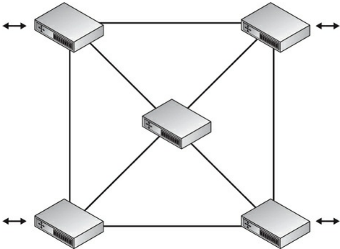
Figure 4-25 In a mesh topology, each node is connected to all other nodes, which provides for redundant paths.
