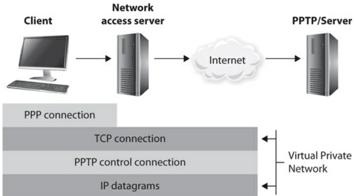
Figure 4-70 PPTP extends PPP connections over IP networks.
