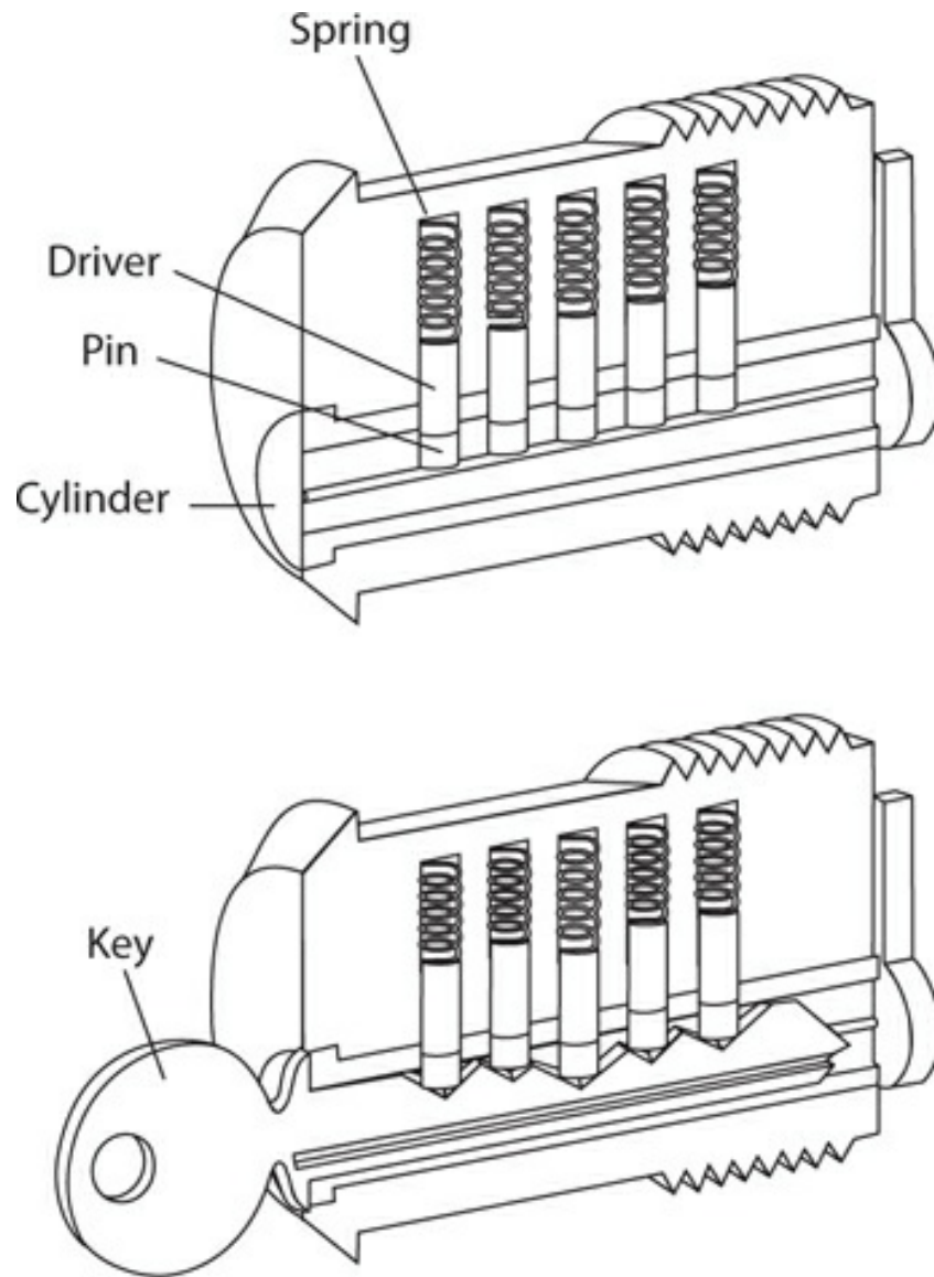
Figure 7-4 Tumbler lock
