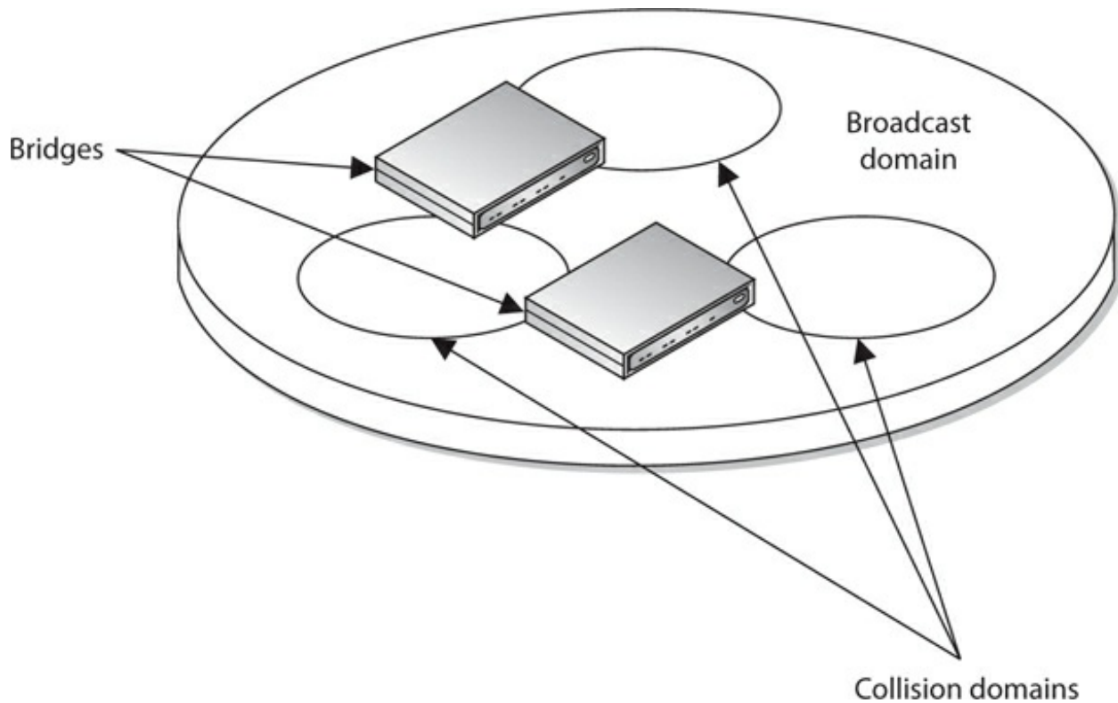
Figure 4-26 Collision domains within one broadcast domain
