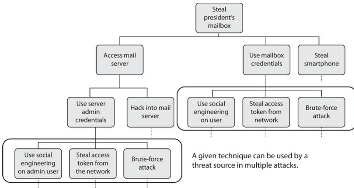
Figure 1-14 A simplified attack tree
