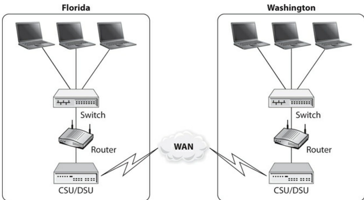
Figure 4-63 A CSU/DSU is required for digital equipment to communicate
