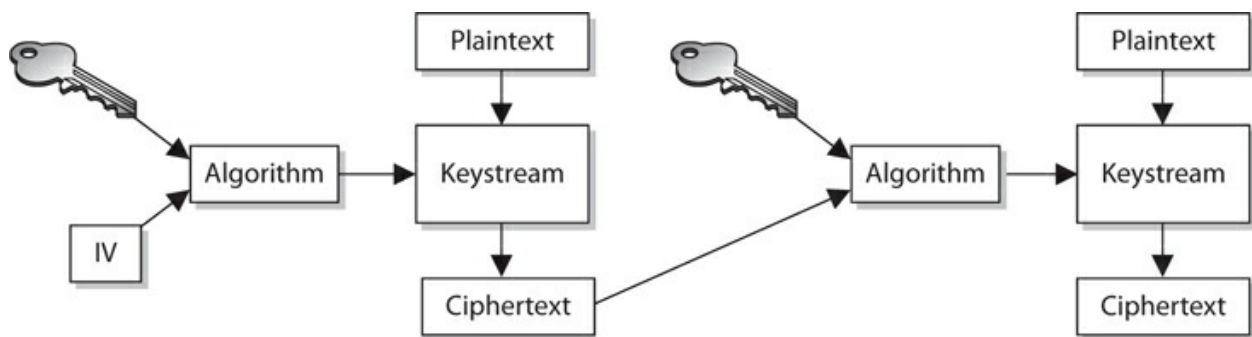
Figure 3-40 A block cipher working in CFB mode
