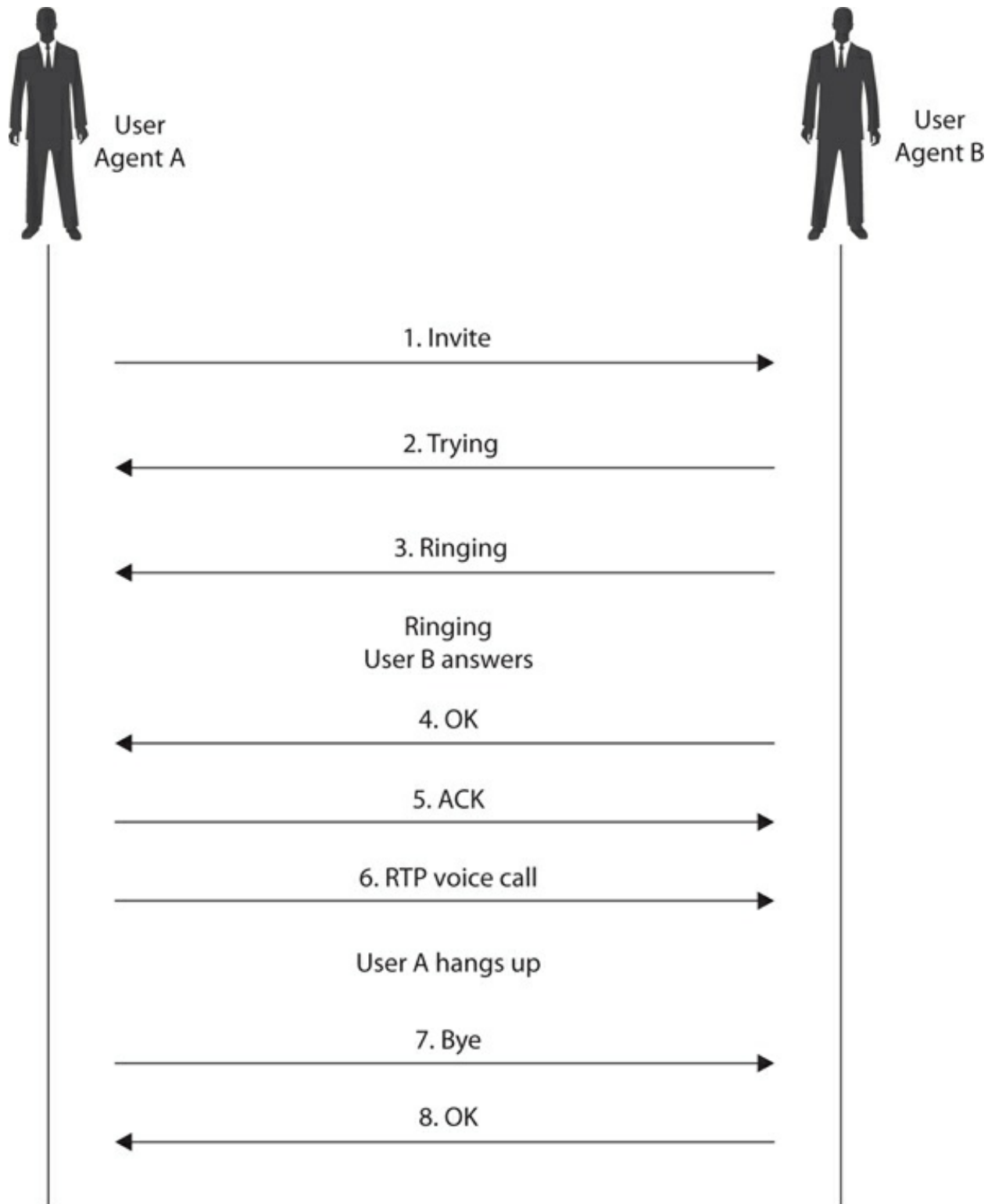
Figure 4-68 SIP handshake
