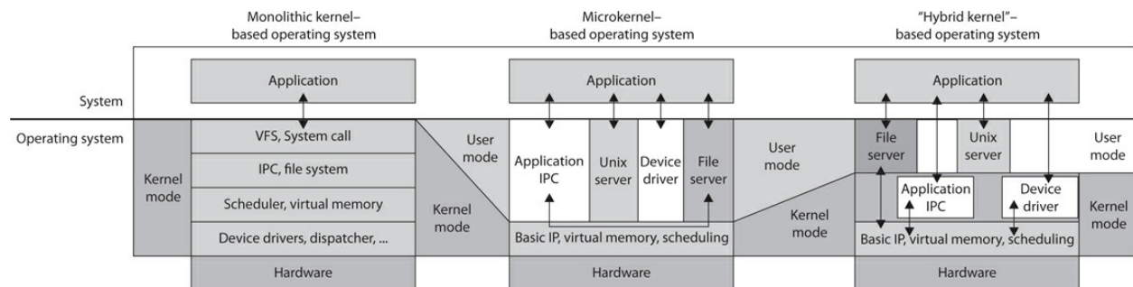
Figure 3-20 Major operating system kernel architectures
