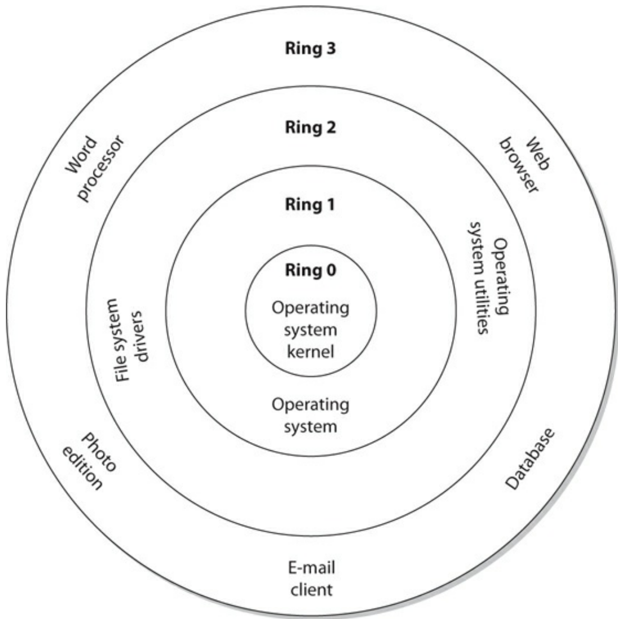
Figure 3-15 More-trusted processes operate within lower-numbered rings.
