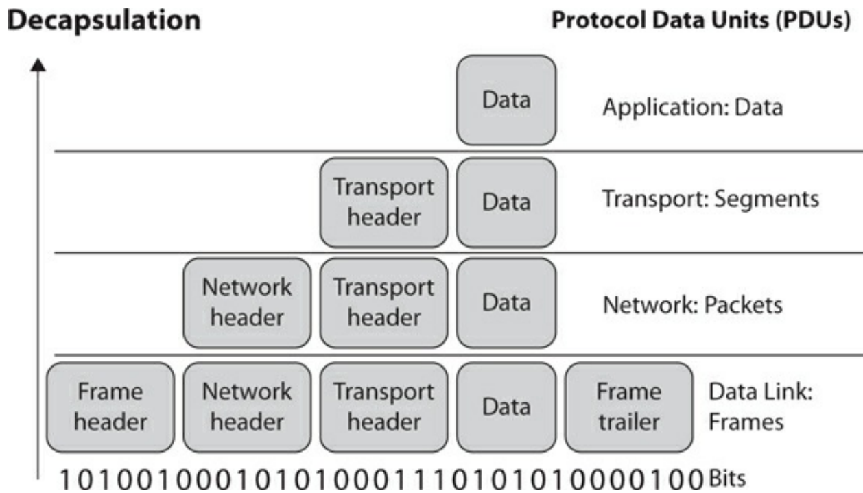
Figure 4-14 Data goes through its own evolutionary stages as it passes through the layers within the network stack.
