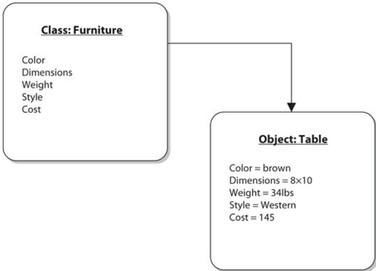
Figure 8-14 In object-oriented inheritance, each object belongs to a class and takes on the attributes of that class
