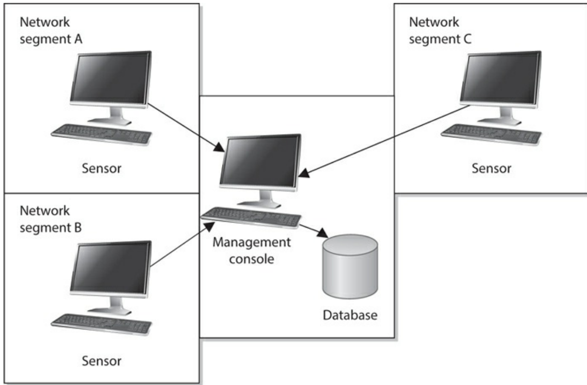
Figure 5-25 Sensors must be placed in each network segment to be monitored by the IDS.
