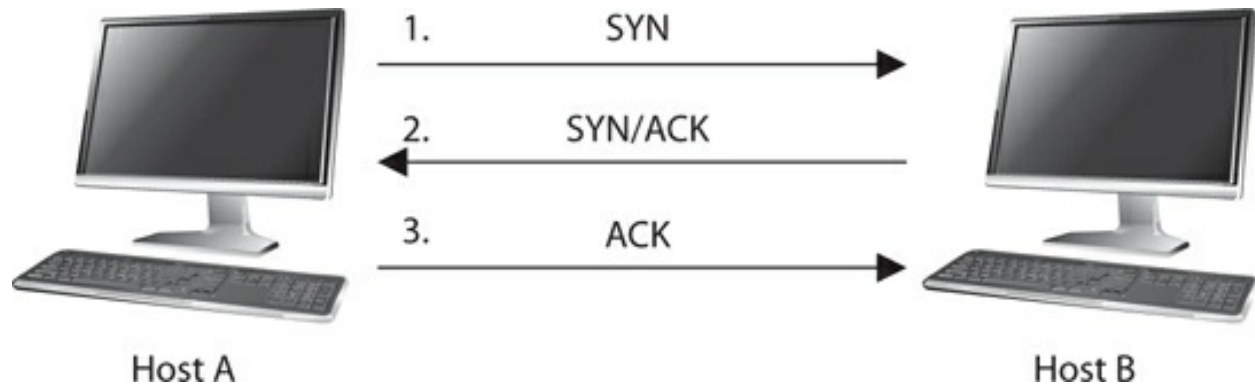
Figure 4-13 The TCP three-way handshake
