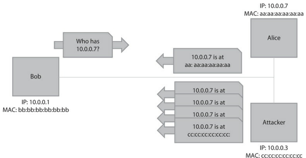
Figure 4-31 ARP poisoning attack
