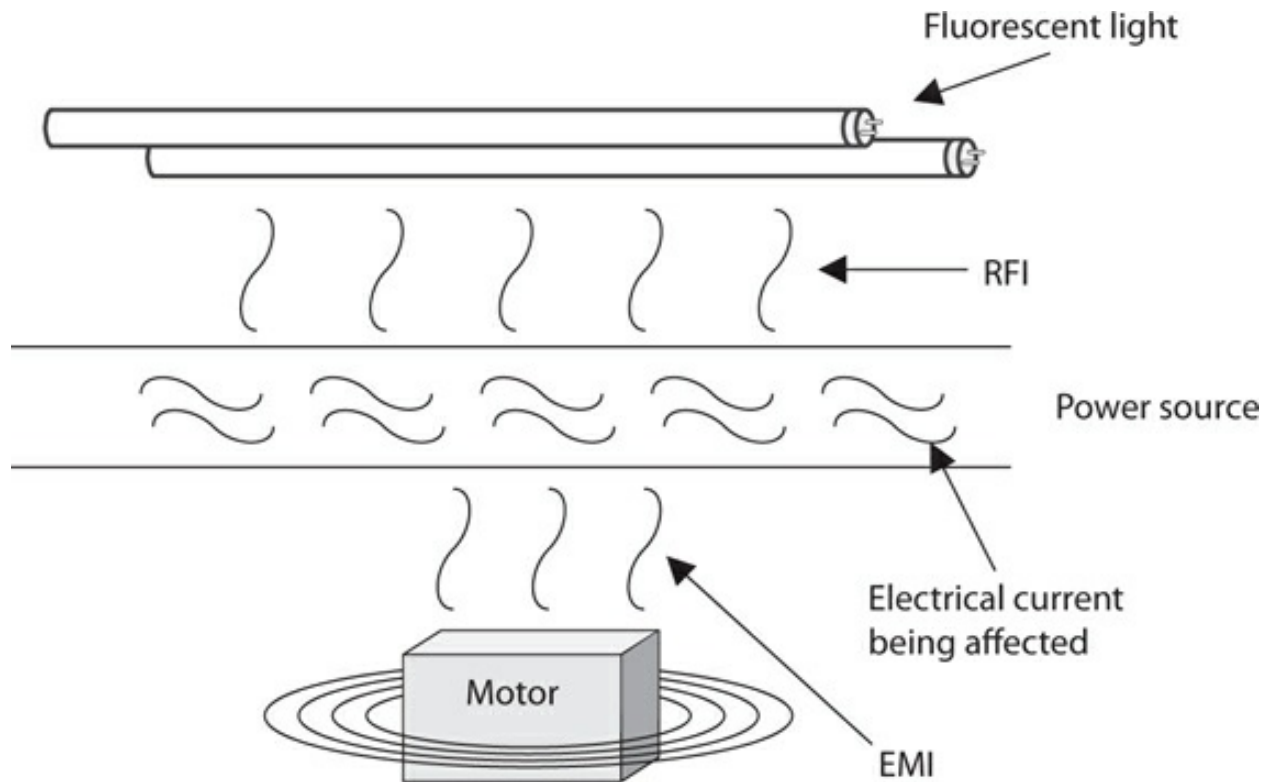
Figure 3-55 RFI and EMI can cause line noise on power lines.
