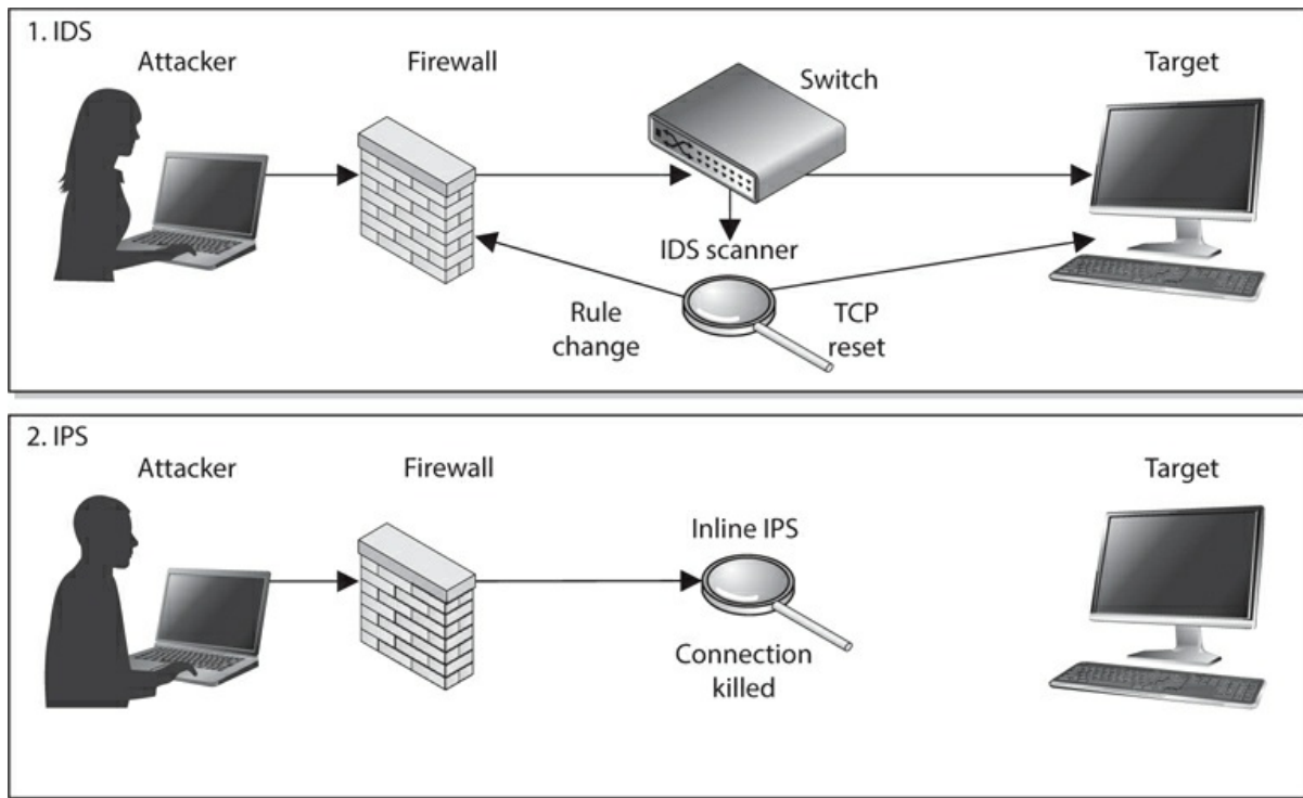
Figure 5-26 IDS vs. IPS architecture
