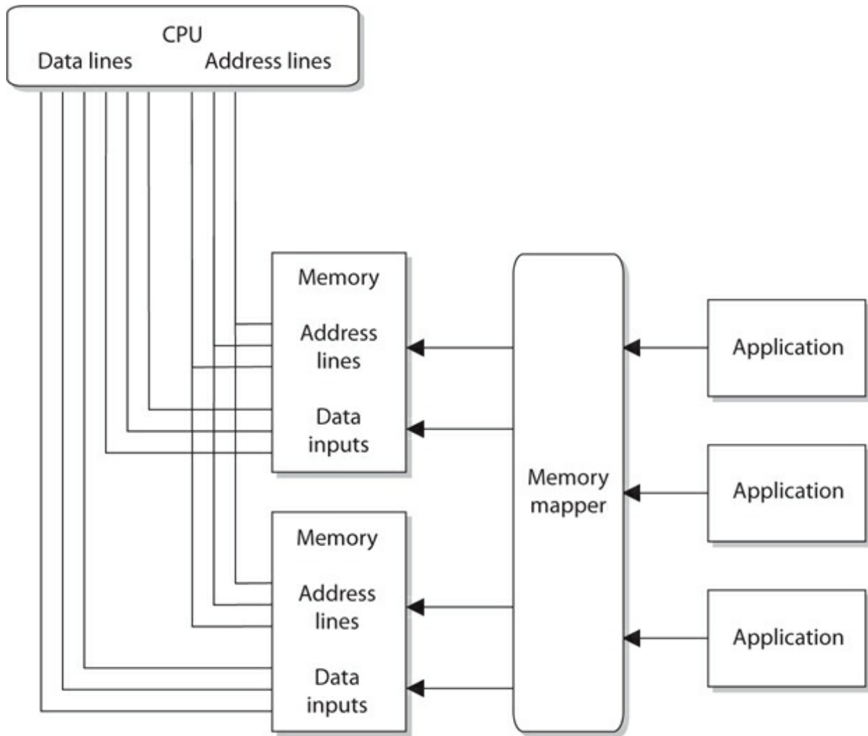
Figure 3-6 The CPU and applications access memory differently.
