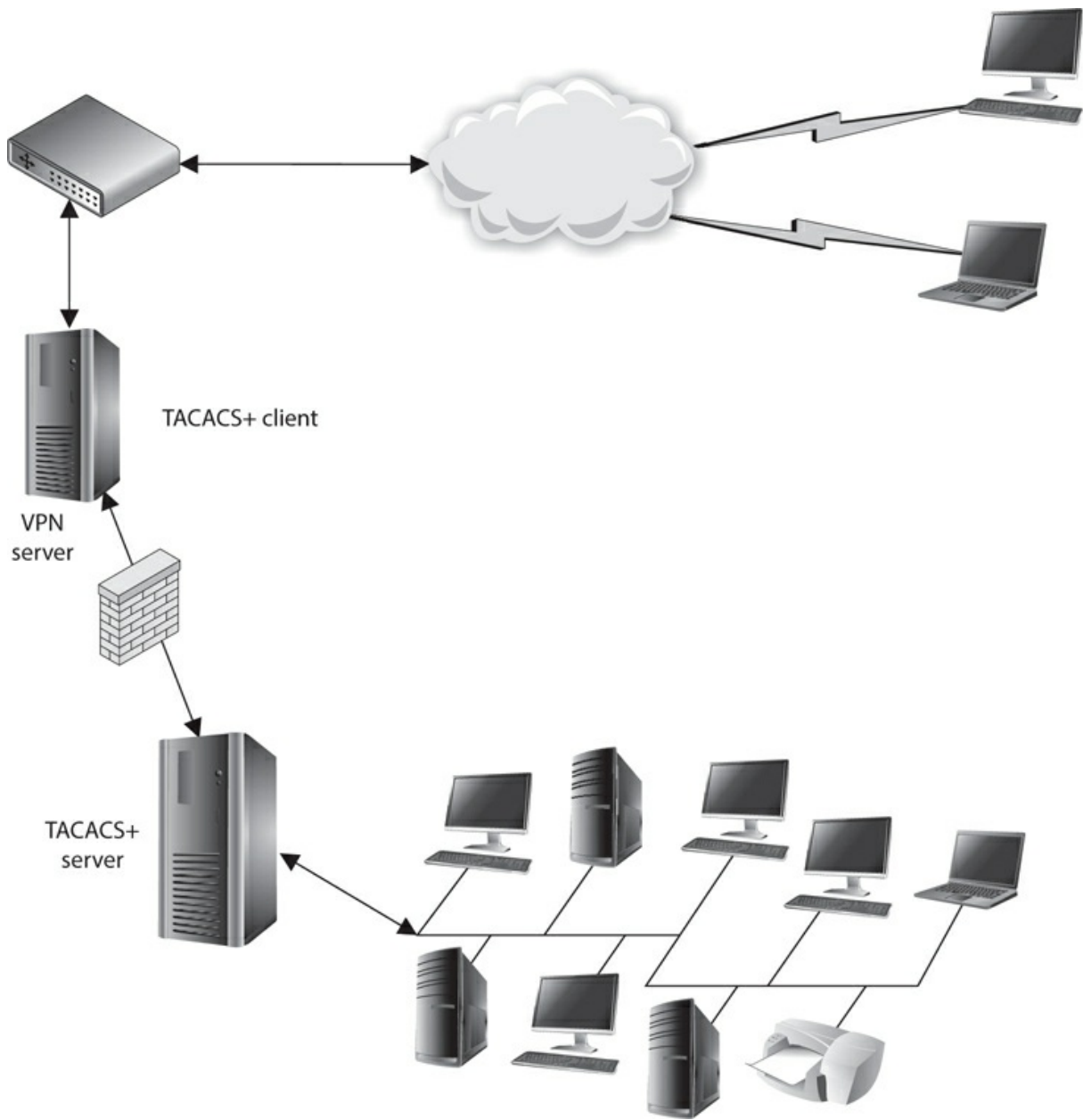
Figure 5-21 TACACS+ works in a client/server model.
