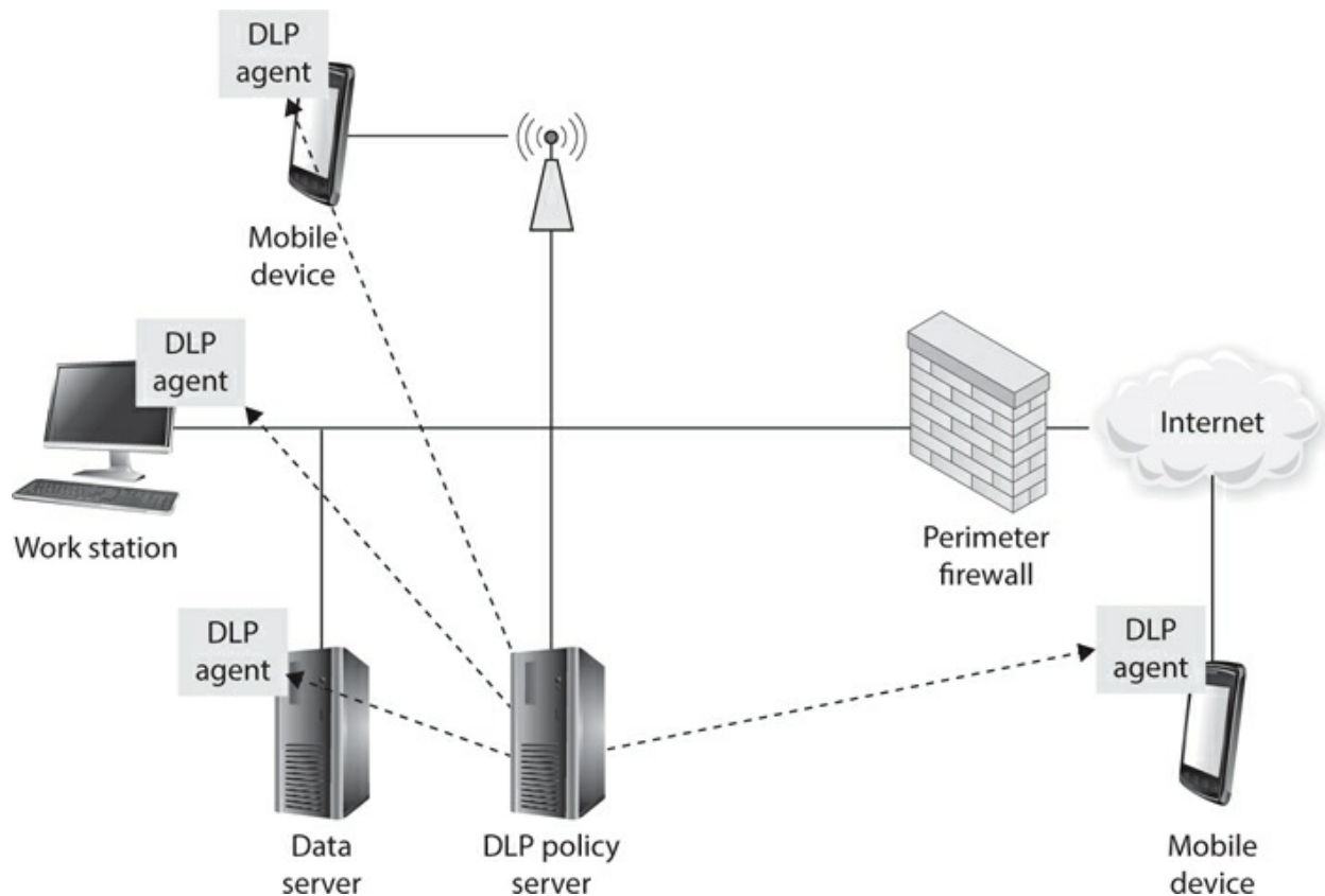
Figure 2-8 Endpoint DLP
