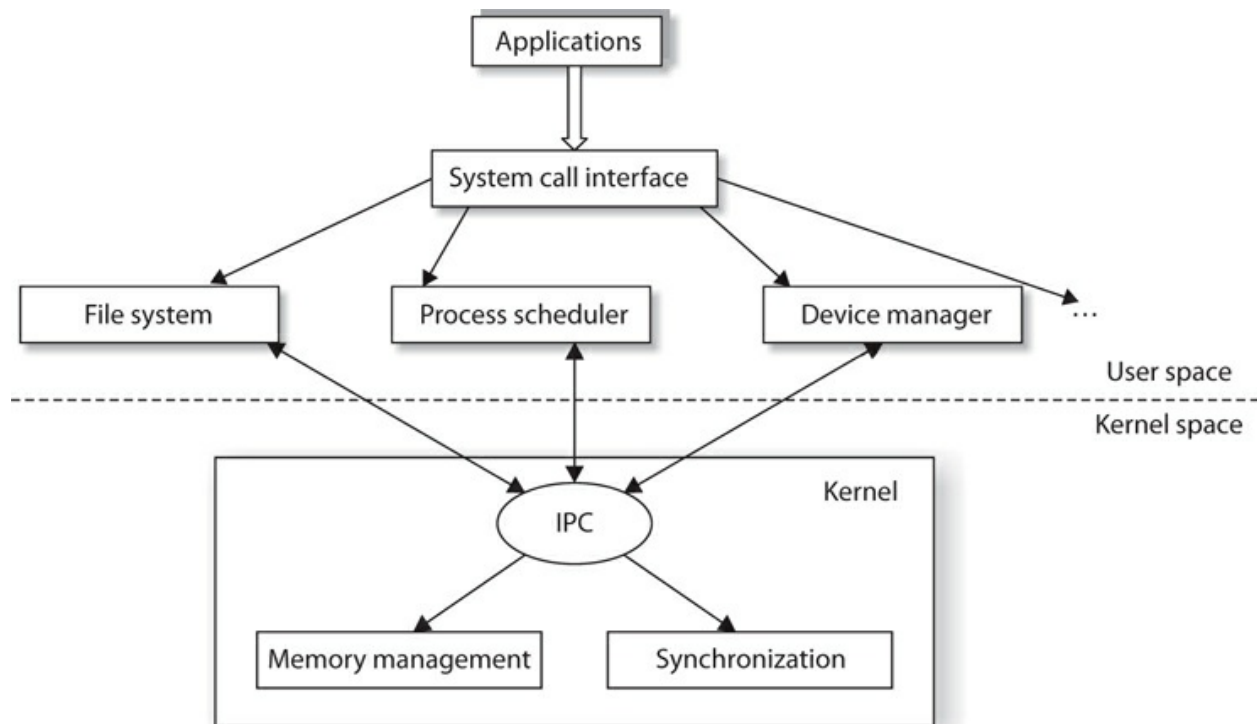
Figure 3-18 Microkernel architecture
