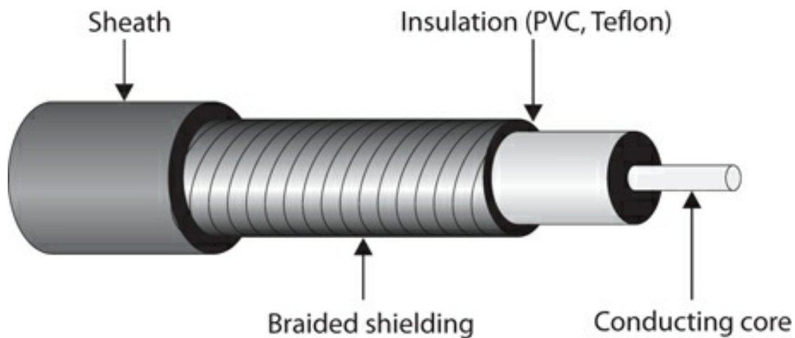
Figure 4-21 Coaxial cable
