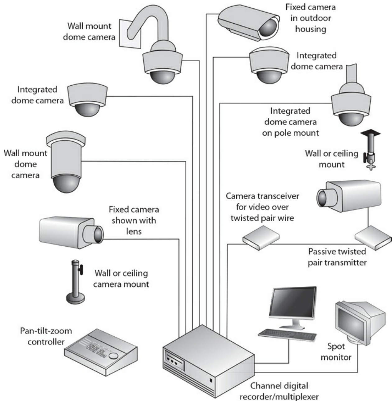
Figure 7-8 A CCTV product can comprise several components.
